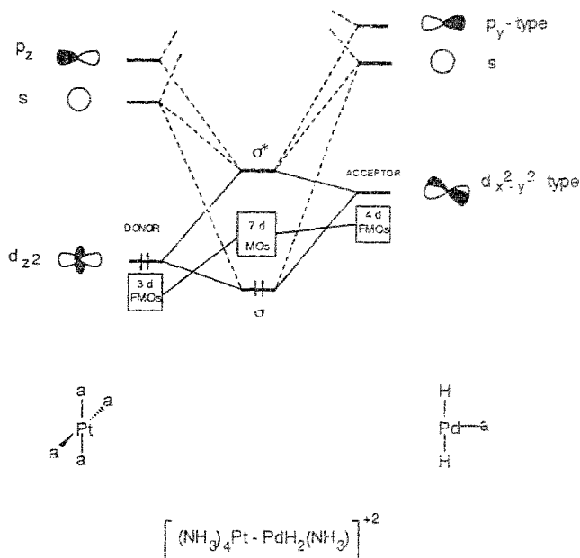
Fig. 13. \text{Pt(II)/d}^8\text{-Pd(II) d}^8 molecular orbital diagram for 4:3 type dimers.
