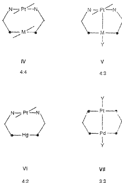
Fig. 9. Trans -dinuclear species 4:4, 4:3, and 4:2 with h-h arrangement of nucleobases. Fragment VII represents dinuclear Pt(II)–Pd(II) species.
