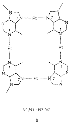
Fig. 18. Hypothesized arrangements for cyclic purine nucleobase quartets.
