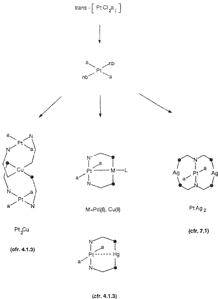
Fig. 6. Concise scheme of species derived from \text{trans-}[(\text{pym})_2\text{Pt}a_2] . The numbers in parentheses refer to the section where the complex is discussed.
