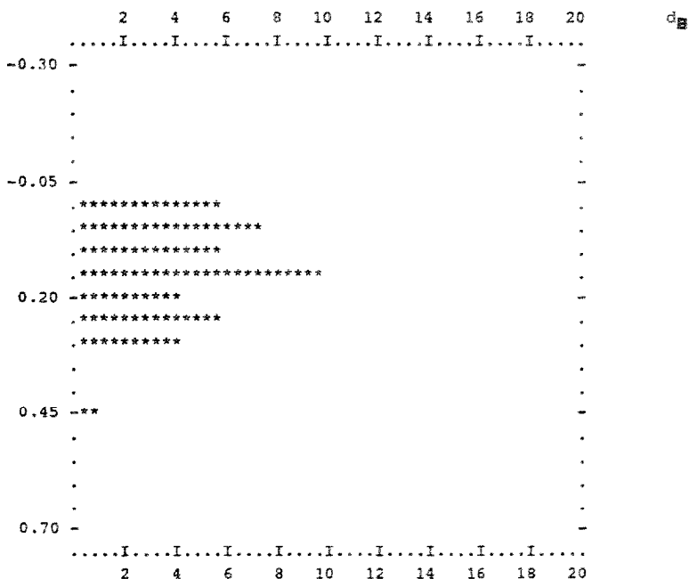
Fig. 21. Histogram for displacement of Pt from pyrimidine ring. d_{\text{Pt}} .
