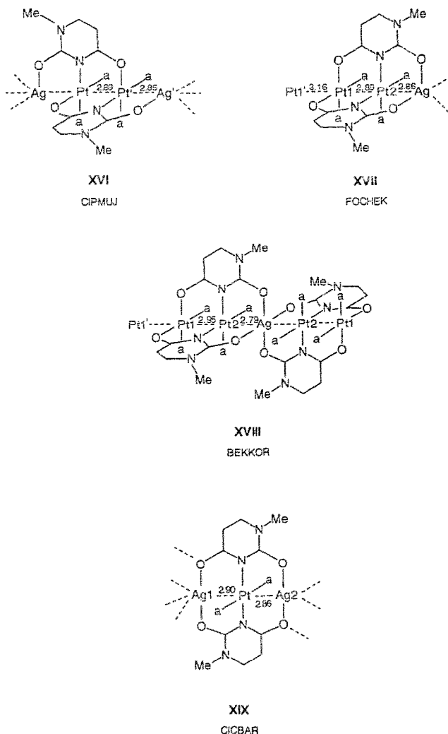
Fig. 16. Polynuclear Pt, Ag complexes so far structurally characterized with metal-metal distances given.
