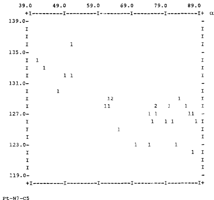
Fig. 4. Plot of angle \alpha against the Pt-N7-C5 bond angle for guanines N7 coordinated.
