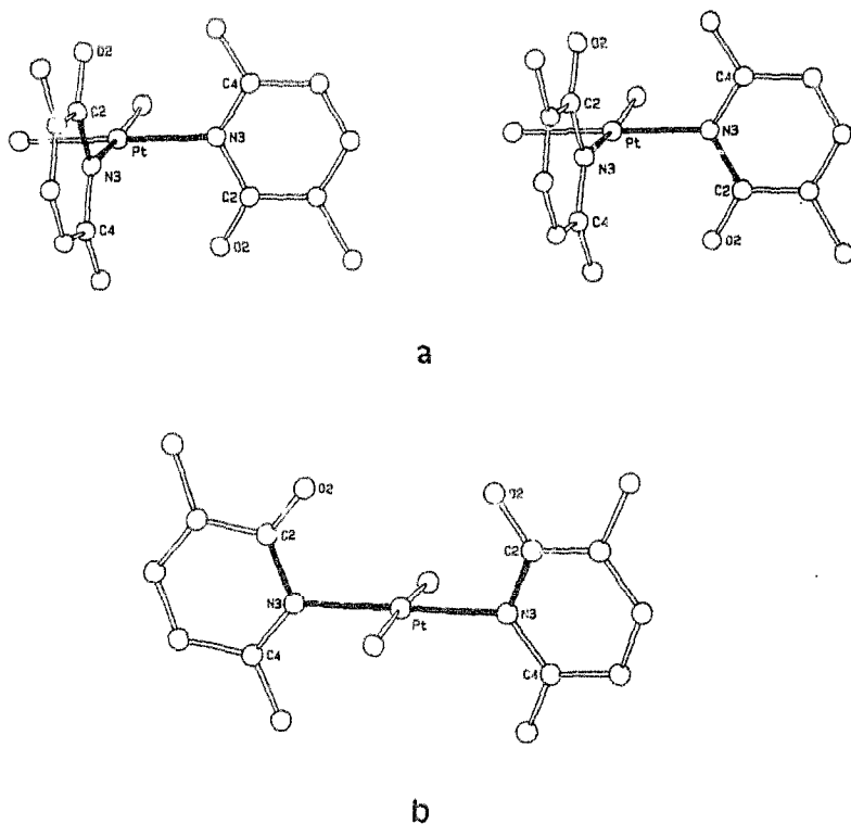
Fig. 3. Torsional angles \phi 1 and \phi 2 defining the bases conformation in cis - and trans -[(nb) 2 Pt] complexes.
