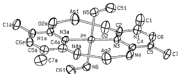
Fig. 17. ORTEP drawing of trinuclear cation \text{trans-[Pt(MeNH}_2)_2\text{Pt(1.5-Me}_2\text{C}^-, \text{O}^{2-}, \text{N}^3, \text{N}^4)\text{Ag}_2]^2+ .
