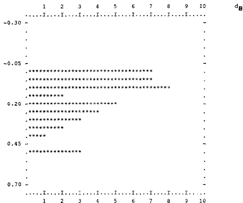
Fig. 22. Histogram for displacement of Pt from a purine ring, d_B .
